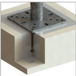
Cast-in CST
